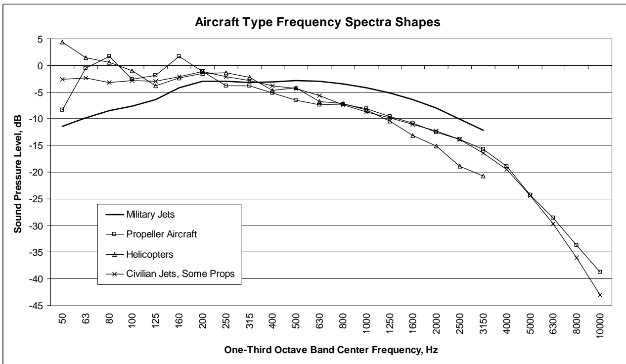
Figure 3-1. Spectra Summary
